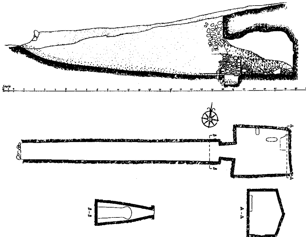
Fig. 4. Dendra tomb 2. (After Persson, Royal tombs , fig. 65.)
